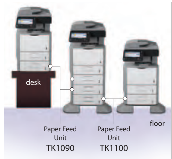
These flexible systems can be configured for desk or floor placement. Stack up to 3 optional Paper Feed Units to boost input capacity to 2,300 sheets.* The Paper Feed Unit TK1100 with casters is designed specifically for floor placement.
